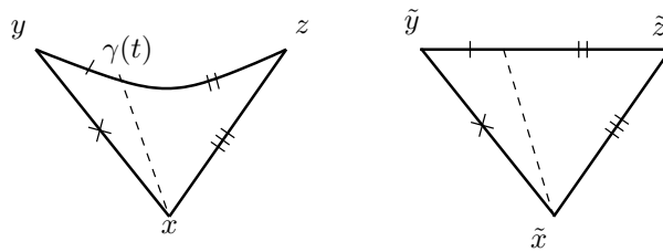
FIGURE 1. The CAT(0) inequality: the dashed segment is shorter in the original triangle on the left than in the comparison triangle on the right.
