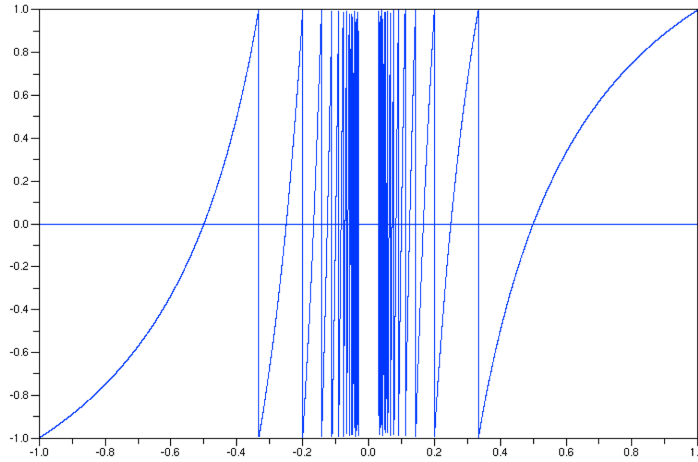
FIGURE 4. The mapping T
