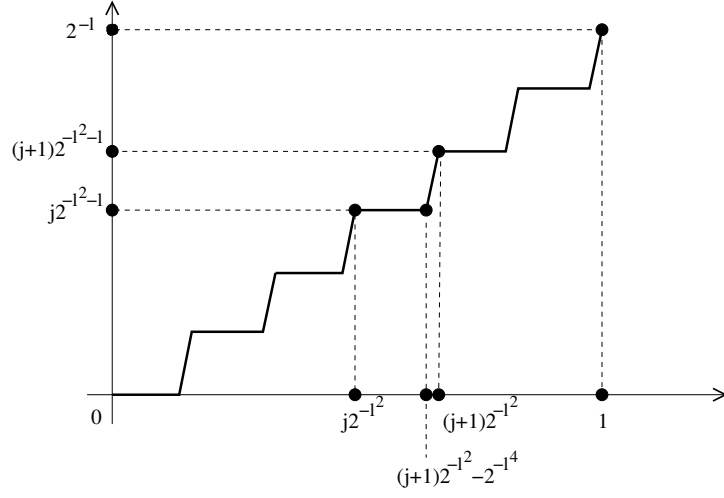
FIGURE 4. Illustration of the graph of the functions \gamma_l
